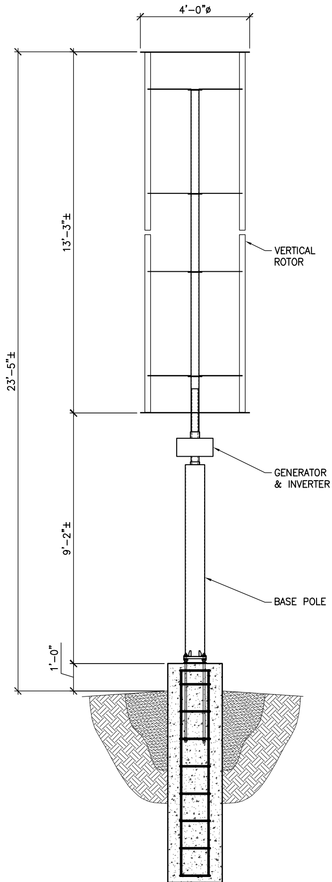
HIGH WIND WINDSPIRE (1.2kW) 30' HT.
